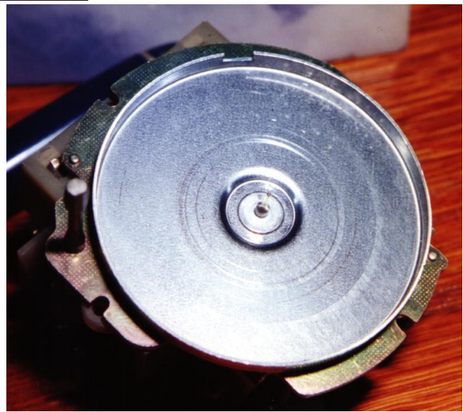
Figure 4. Now the odometer wheel frame has been removed from the magnet wheel frame. This is a view of the underside of the odometer wheel frame with the attached drag cup. In the center of the drag cup is the thin spindle which fits into the bushing in the center of the magnet wheel.
