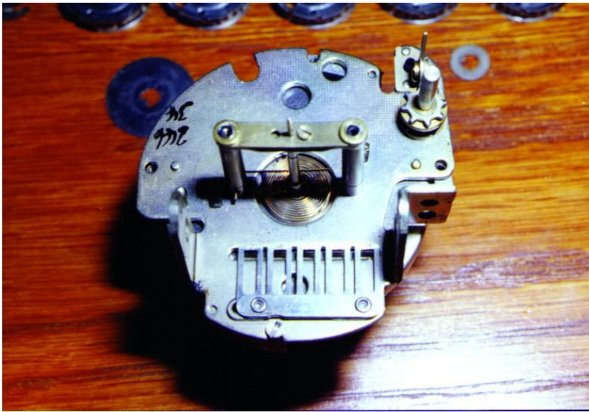
Figure 9. The main frame of the "Early" speedometer with the main odometer disassembled and the trip odometer frame removed. The "hair spring" is visible. On the other side of the frame is the drag cup. This frame is from an MGA and has the trip reset wheel entering straight into the frame. The metal fingers which allow indexing of the odometer wheels are visible on the lower section of the frame.
