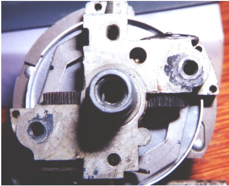
Figure 18. A view of the rear of an old-style speedometer. Note the twin 32 tooth worm gears. One for each wheel set.
