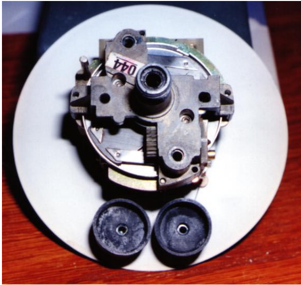
Figure 12. This is from a TR6 (New-style). Viewed from the rear with the case removed. You can see the input shaft in the center. You also see the grey plastic gear which is driven off the worm. Also visible here are the magnet wheel and the drag cup (silver ). These will be shown in greater detail in upcoming photographs.
