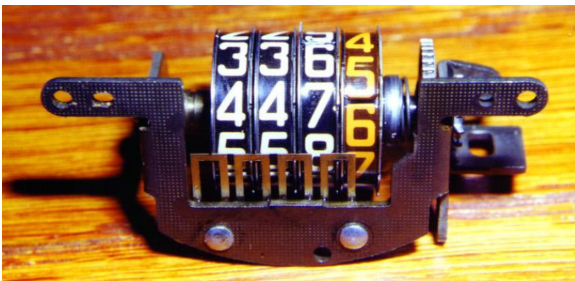
Figure 11. An "early" trip odometer incorporating wheels identical to the main odometer. The trip odometer is mounted on its own sub-frame. The metal fingers are shown holding the wheels. It is clear how each wheel can release the finger restraining the wheel to the left.
