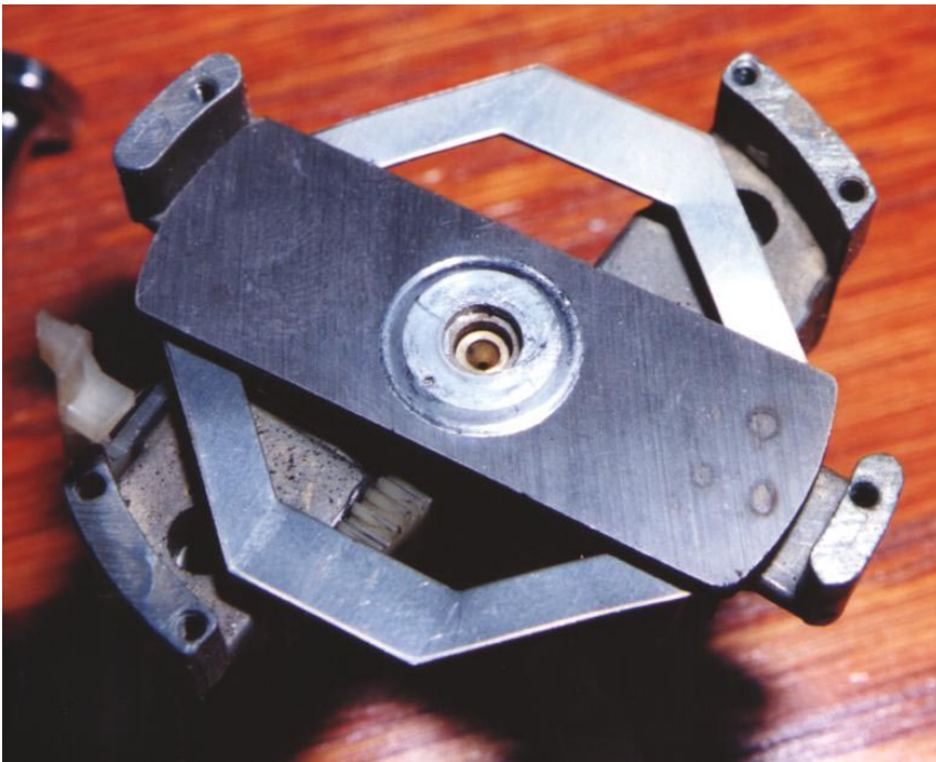
Figure 5. This is a view of the front of the magnet wheel after removal of the odometer wheel frame. In the center is the brass bushing in which the spindle of the pointer rides.
