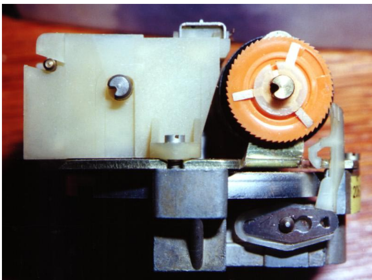
Figure 14. A view of the left side of the same speedometer. You can see the orange speedometer drive gear, the grey plastic retaining washer, the white plastic pawl which pushes the drive gear, and the dark metal retaining clip on the base of the pawl.
