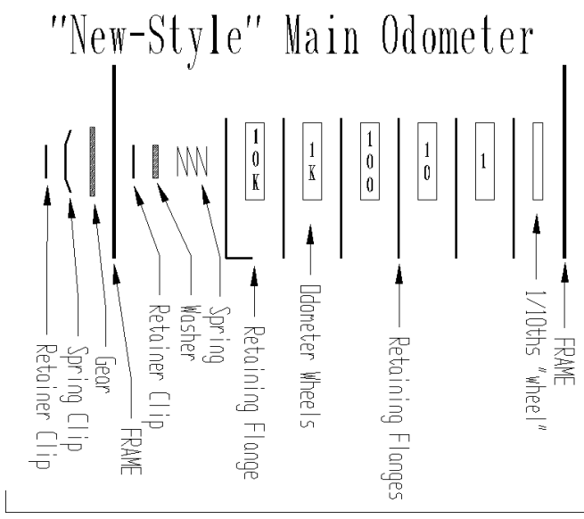
Figure 8. Diagram of "new-style" odometer components
