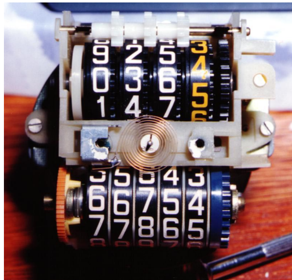
Figure 14. A view of the left side of the same speedometer. You can see the orange speedometer drive gear, the grey plastic retaining washer, the white plastic pawl which pushes the drive gear, and the dark metal retaining clip on the base of the pawl.
