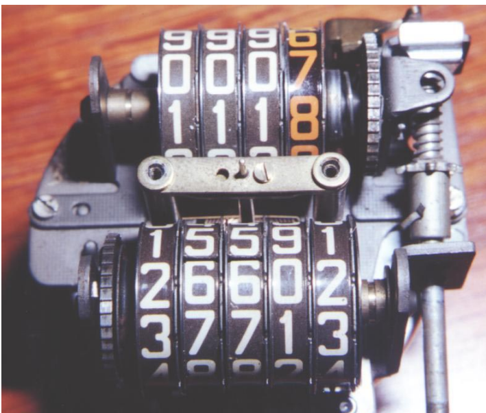
Figure 17. A view of the front of an "Old-style" speedometer. Note the separate odometer drive gears for each wheel set. Also note the all metal construction. The trip odometer wheels are set immediately next to each other in contrast to later speedometers such as the new-style one in the earlier photographs (fig. 2). The shaft on the right is the trip odometer reset. The return spring is not in the same place as the later speedometer. It is just above the pointer under the odometer wheels.
