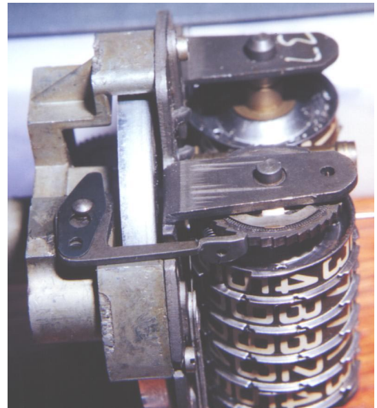
Figure 19. A view of the left of an old-style speedometer.. Note the all-metal construction. The shiny thin metal against the left side of the odometer drive gear is the combination retaining washer/ratcheting lock. The number "37" written (by the manufacturer) on the frame is the number of teeth on the odometer drive gears.
