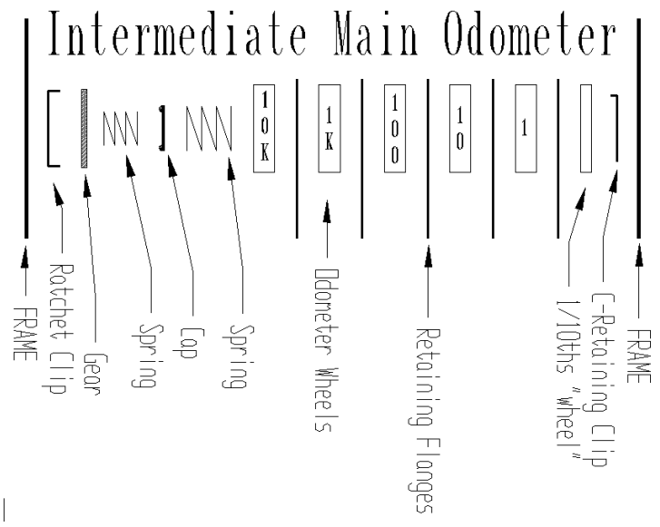
Figure 8. Diagram of "new-style" odometer components
