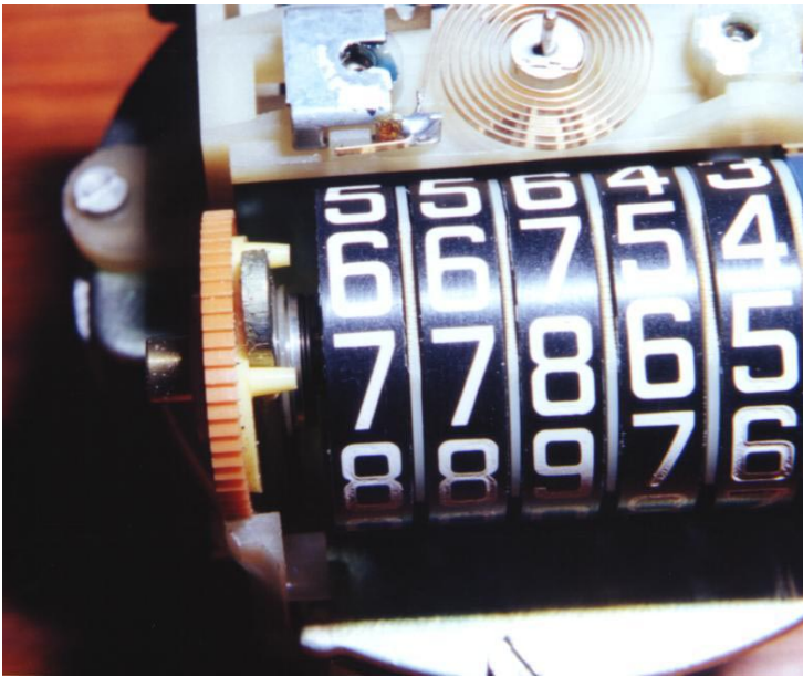
Figure 15. A close up of the front of the odometer drive gear. The yellow plastic legs to the right of the gear are attached to a plastic which has a splined surface and provided a ratcheting action to the gear. The legs prevent rotation of the yellow . Just to the right of the metal arm of the frame you can see the egde of a second grey plastic retaining washer.
