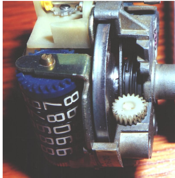
Figure 17. A view of the front of an "Old-style" speedometer. Note the separate odometer drive gears for each wheel set. Also note the all metal construction. The trip odometer wheels are set immediately next to each other in contrast to later speedometers such as the new-style one in the earlier photographs (fig. 2). The shaft on the right is the trip odometer reset. The return spring is not in the same place as the later speedometer. It is just above the pointer under the odometer wheels.
